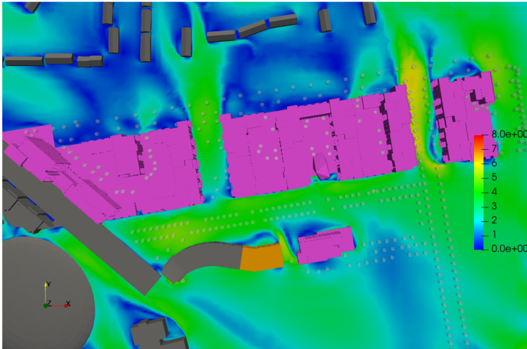
Figure 6.8: Ground Floor Level - Flow Velocity Results at Z=1.5m above the ground including existing buildings (in grey) and permitted but not constructed (in orange) - Wind Direction: 135°
