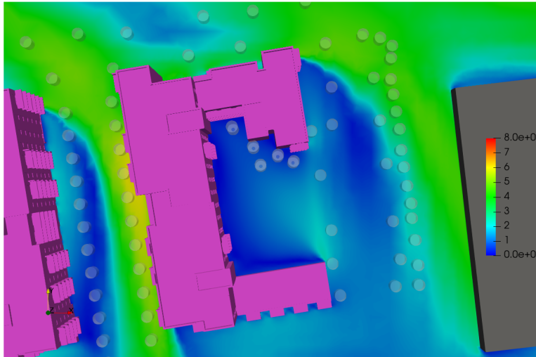
Figure 6.44: Block F Podium - Flow Velocity Results at Z=1.5m above the Podium - Wind Direction: 315°
