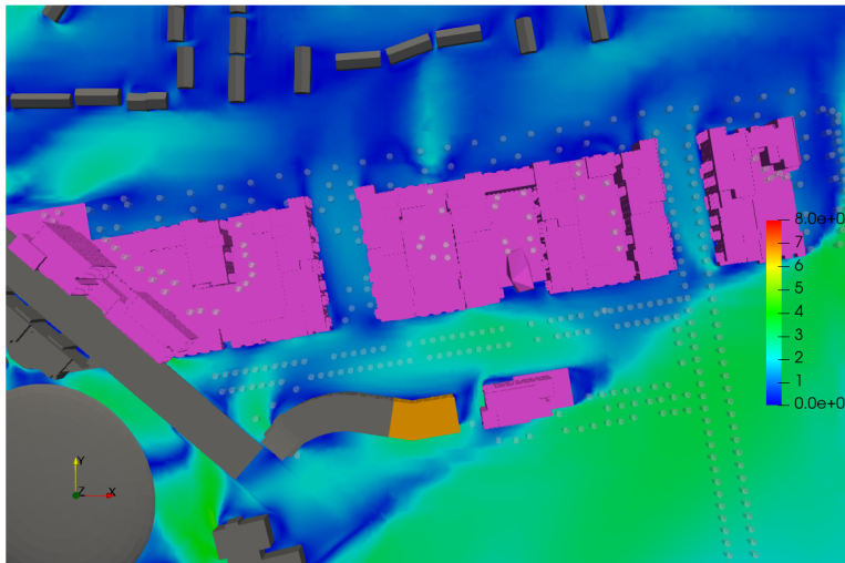
Figure 6.6: Ground Floor Level - Flow Velocity Results at Z=1.5m above the ground including existing buildings (in grey) and permitted but not constructed (in orange) - Wind Direction: 225°
