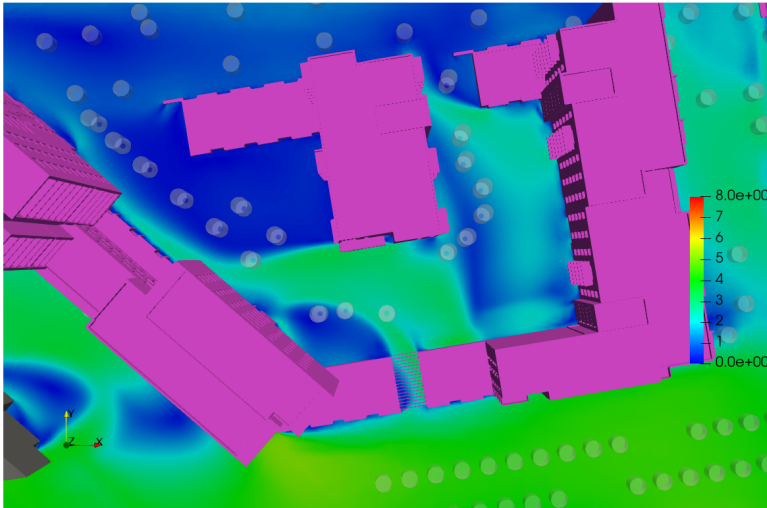
Figure 6.24: Block A/B/C Podium - Flow Velocity Results at Z=1.5m above the Podium - Wind Direction: 236°
