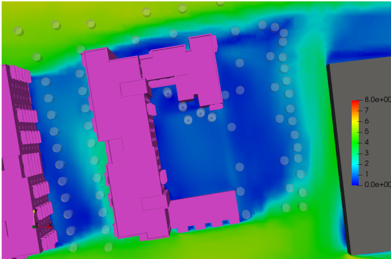
Figure 6.41: Block F Podium - Flow Velocity Results at Z=1.5m above the Podium - Wind Direction: 258°
