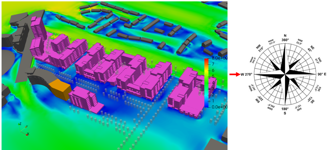
Figure 6.17: Wind Speed Results at 1.5m Above Development Ground Floor including existing buildings (in grey) and permitted but not constructed (in orange) - 3D View - Wind Direction: 270°
