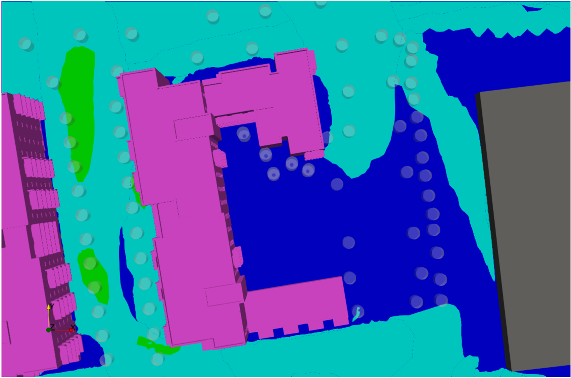
Figure 6.67: Block F Podium - Lawson Discomfort Map - Top View
