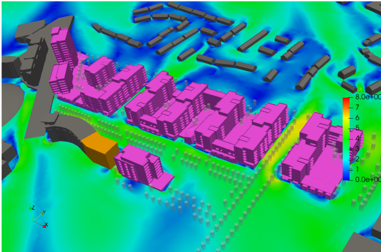
Figure 6.9: Wind Speed Results at 1.5m Above Development Ground Floor including existing buildings (in grey) and permitted but not constructed (in orange) - 3D View - Wind Direction: 135°
