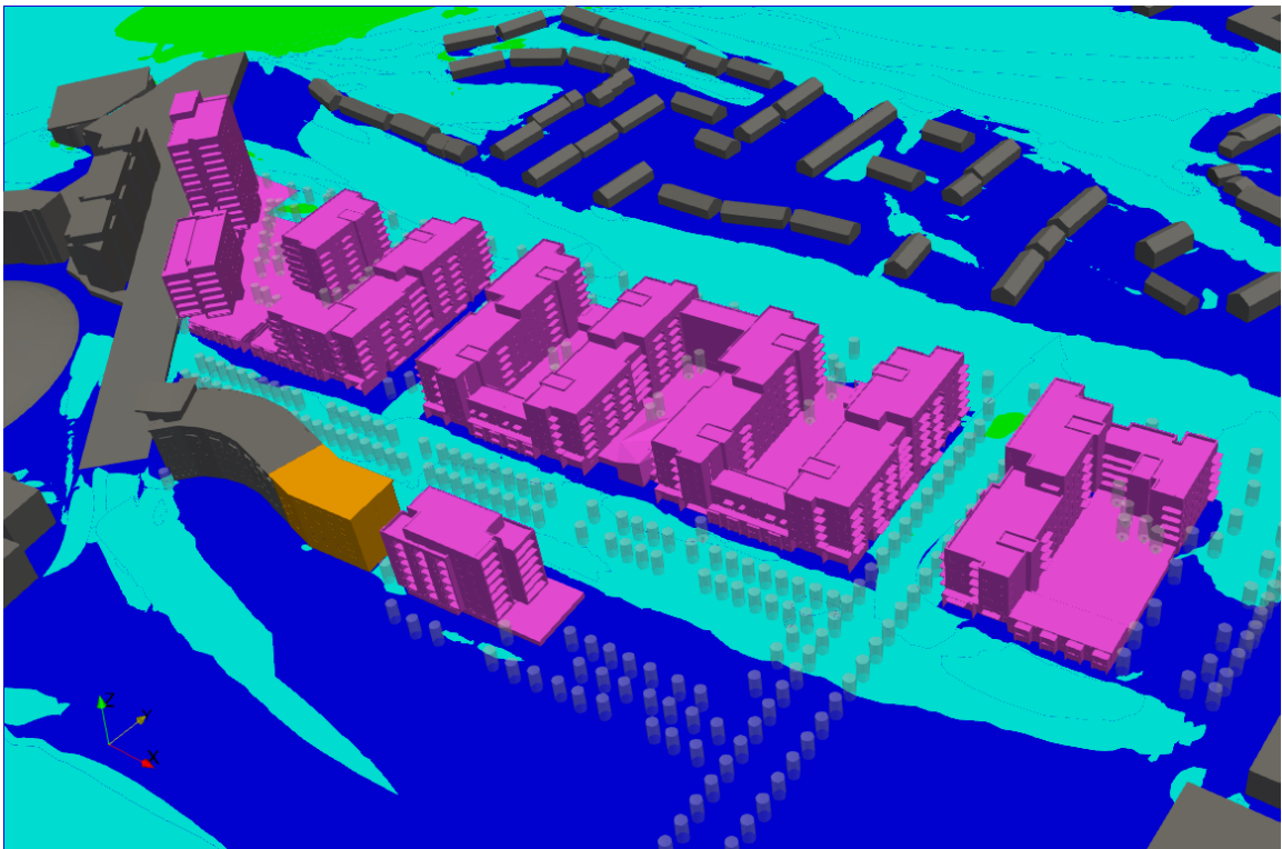
Figure 6.64: Ground Floor - Lawson Discomfort Map - 3D view
