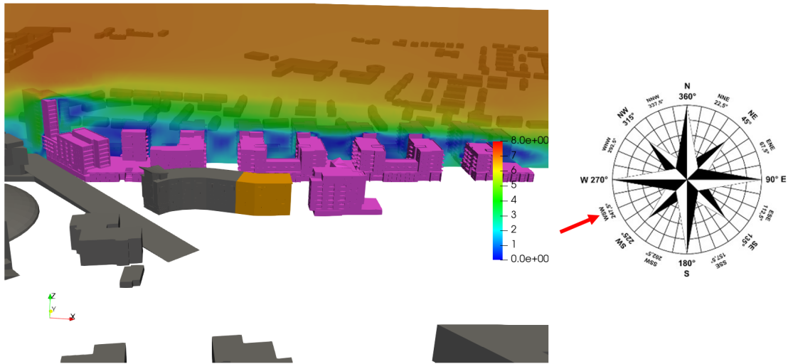
Figure 6.54: Flow Velocity Results of some balconies on the West/East sides of the development - Wind Direction: 247°
