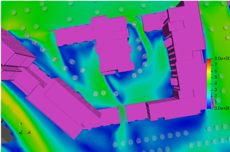
Figure 6.28: Block A/B/C Podium - Flow Velocity Results at Z=1.5m above the Podium - Wind Direction: 315°
