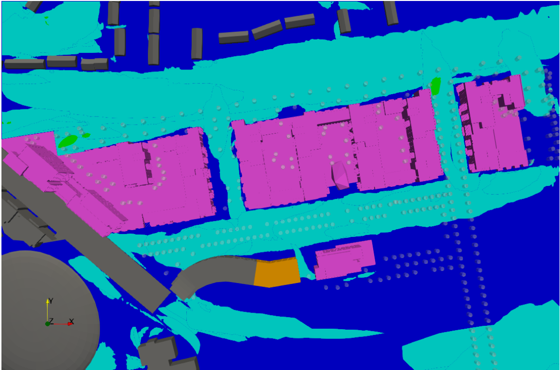
Figure 6.63: Ground Floor - Lawson Discomfort Map - Top View
