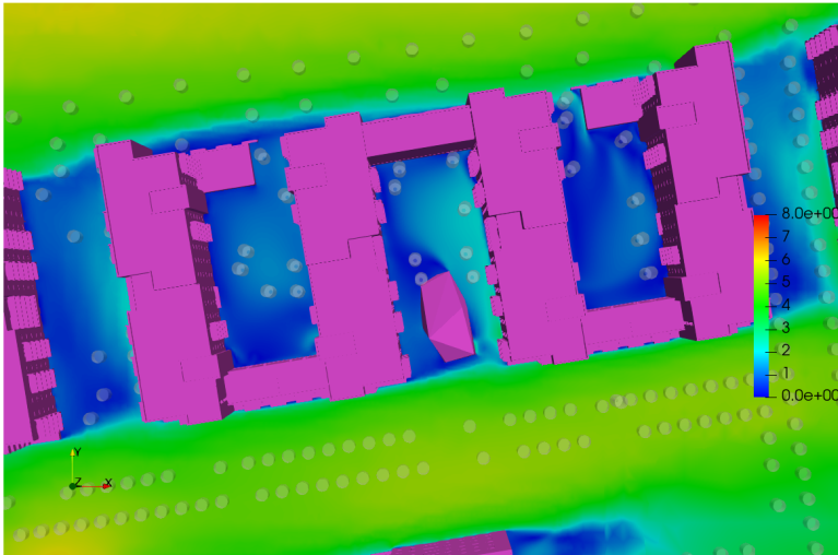
Figure 6.33: Block D/E Podium - Flow Velocity Results at Z=1.5m above the Podium - Wind Direction: 258°
