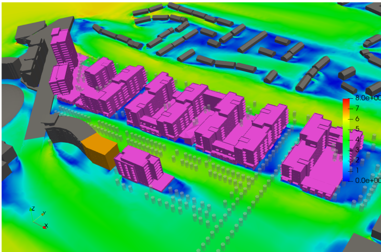
Figure 6.13: Wind Speed Results at 1.5m Above Development Ground Floor including existing buildings (in grey) and permitted but not constructed (in orange) - 3D View - Wind Direction: 258°
