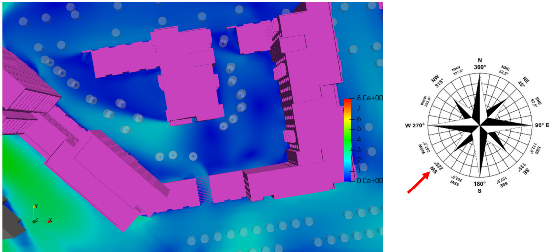
Figure 6.22: Block A/B/C Podium - Flow Velocity Results at Z=1.5m above the Podium - Wind Direction: 225°
