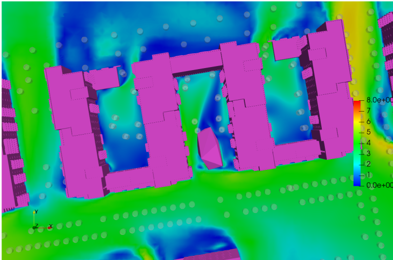
Figure 6.31: Block D/E Podium - Flow Velocity Results at Z=1.5m above the Podium - Wind Direction: 135°
