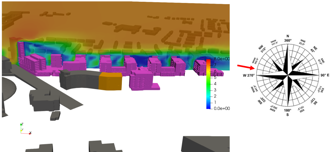
Figure 6.60: Flow Velocity Results of some balconies on the West/East sides of the development - Wind Direction: 281°
