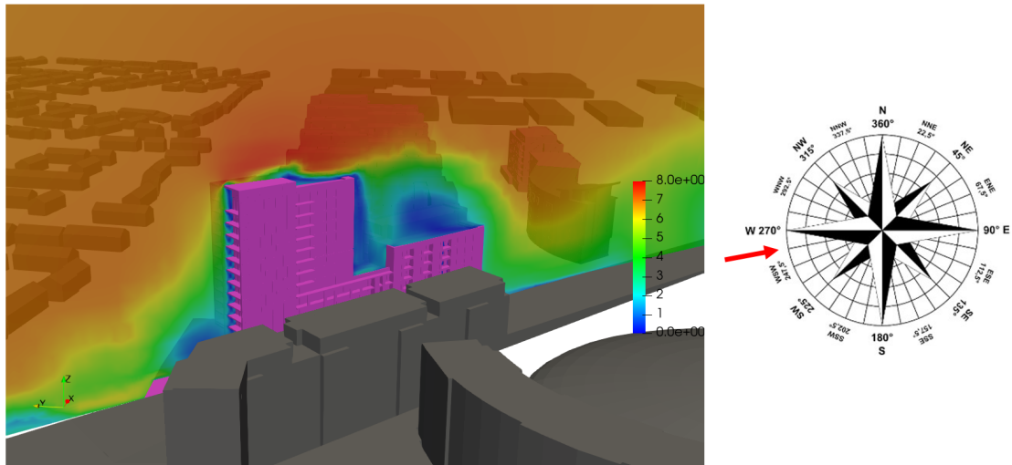
Figure 6.53: Flow Velocity Results of some balconies on the tallest building of the development - Wind Direction: 258°
