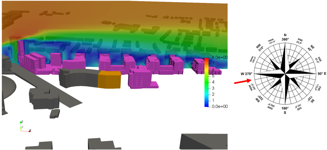
Figure 6.52: Flow Velocity Results of some balconies on the West/East sides of the development - Wind Direction: 258°
