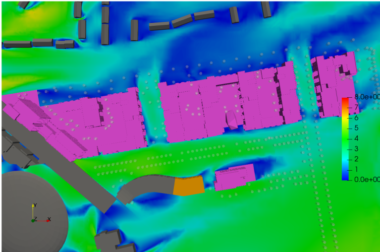
Figure 6.10: Ground Floor Level - Flow Velocity Results at Z=1.5m above the ground including existing buildings (in grey) and permitted but not constructed (in orange) - Wind Direction: 236°
