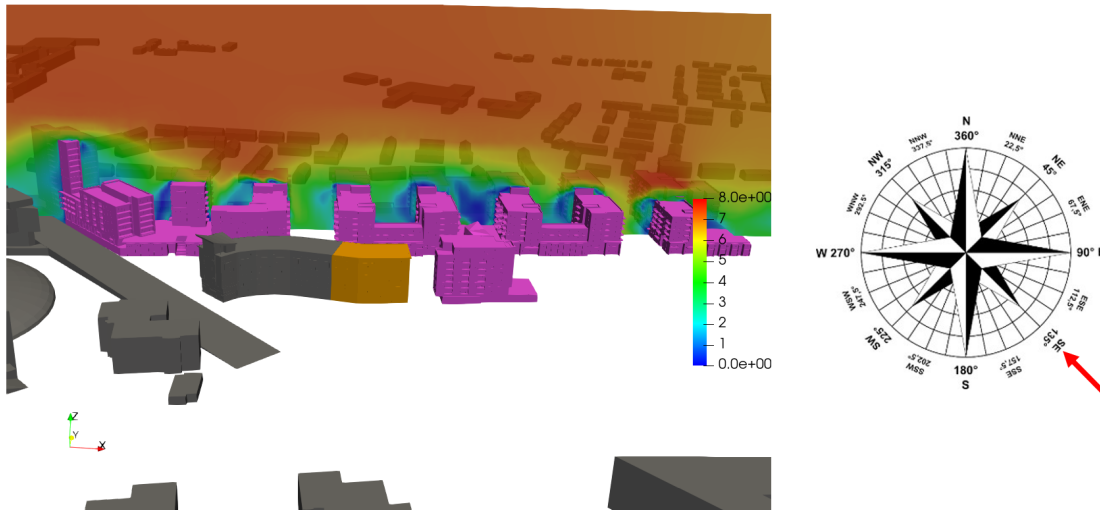
Figure 6.48: Flow Velocity Results of some balconies on the West/East sides of the development - Wind Direction: 135°
