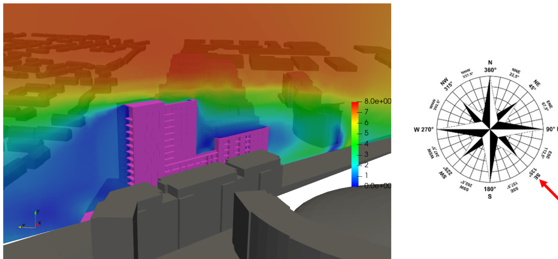
Figure 6.49: Flow Velocity Results of some balconies on the tallest building of the development - Wind Direction: 135°
