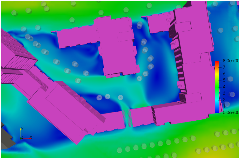
Figure 6.25: Block A/B/C Podium - Flow Velocity Results at Z=1.5m above the Podium - Wind Direction: 258°
