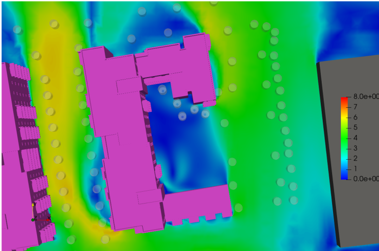
Figure 6.39: Block F Podium - Flow Velocity Results at Z=1.5m above the Podium - Wind Direction: 135°
