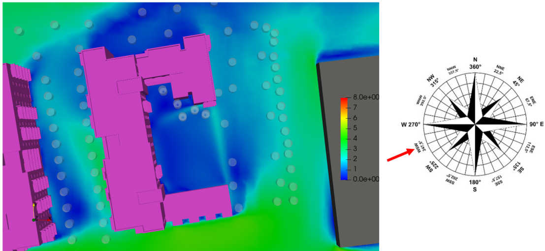
Figure 6.42: Block F Podium - Flow Velocity Results at Z=1.5m above the Podium - Wind Direction: 247°
