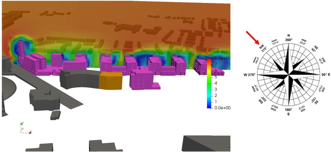
Figure 6.58: Flow Velocity Results of some balconies on the West/East sides of the development - Wind Direction: 315°
