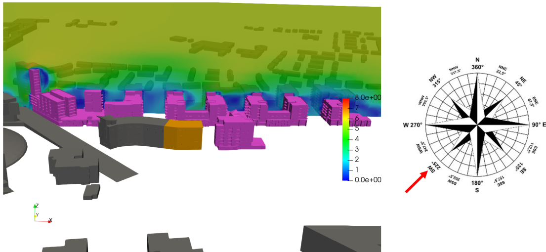
Figure 6.46: Flow Velocity Results of some balconies on the West/East sides of the development - Wind Direction: 225°
