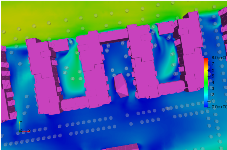
Figure 6.35: Block D/E Podium - Flow Velocity Results at Z=1.5m above the Podium - Wind Direction: 270°
