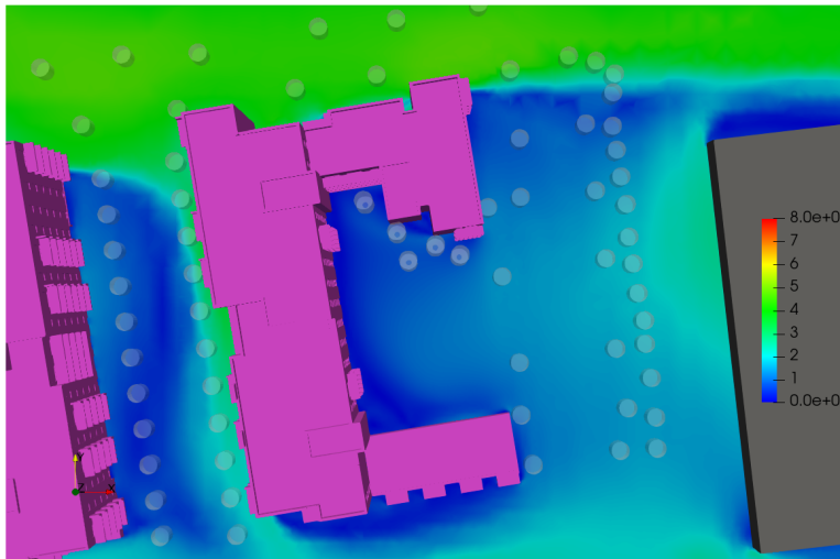
Figure 6.45: Block F Podium - Flow Velocity Results at Z=1.5m above the Podium - Wind Direction: 281°
