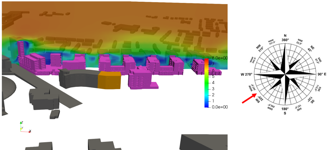
Figure 6.50: Flow Velocity Results of some balconies on the West/East sides of the development - Wind Direction: 236°
