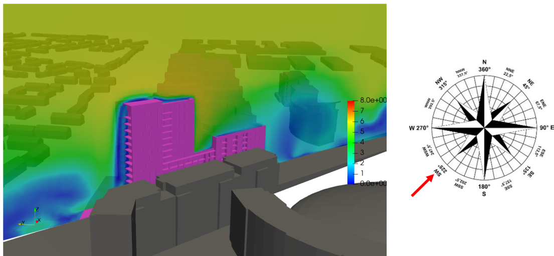
Figure 6.47: Flow Velocity Results of some balconies on the tallest building of the development - Wind Direction: 225°
