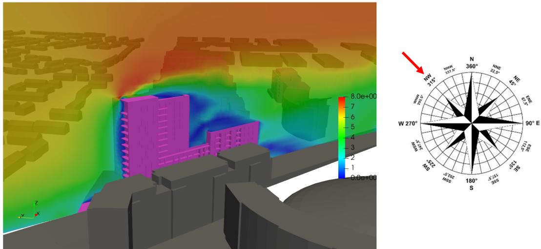
Figure 6.59: Flow Velocity Results of some balconies on the tallest building of the development - Wind Direction: 315°
