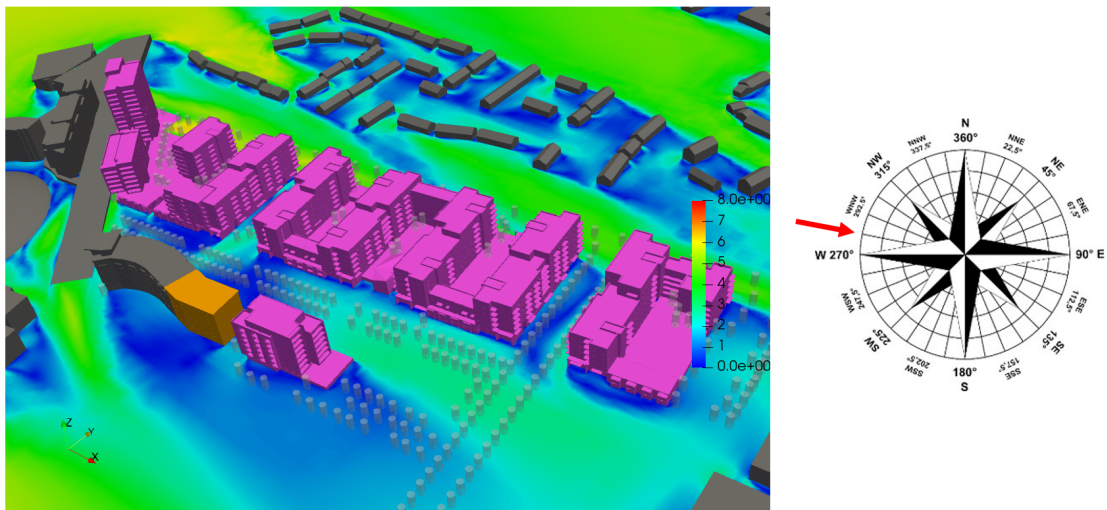
Figure 6.21: Wind Speed Results at 1.5m Above Development Ground Floor including existing buildings (in grey) and permitted but not constructed (in orange) - 3D View - Wind Direction: 281°
