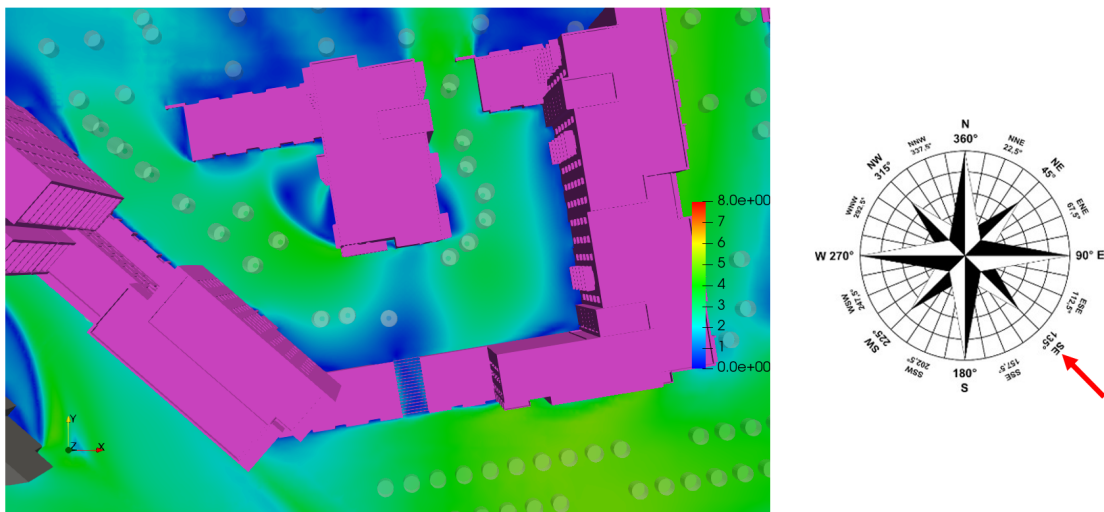
Figure 6.23: Block A/B/C Podium - Flow Velocity Results at Z=1.5m above the Podium - Wind Direction: 135°
