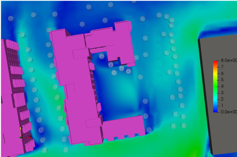
Figure 6.40: Block F Podium - Flow Velocity Results at Z=1.5m above the Podium - Wind Direction: 236°
