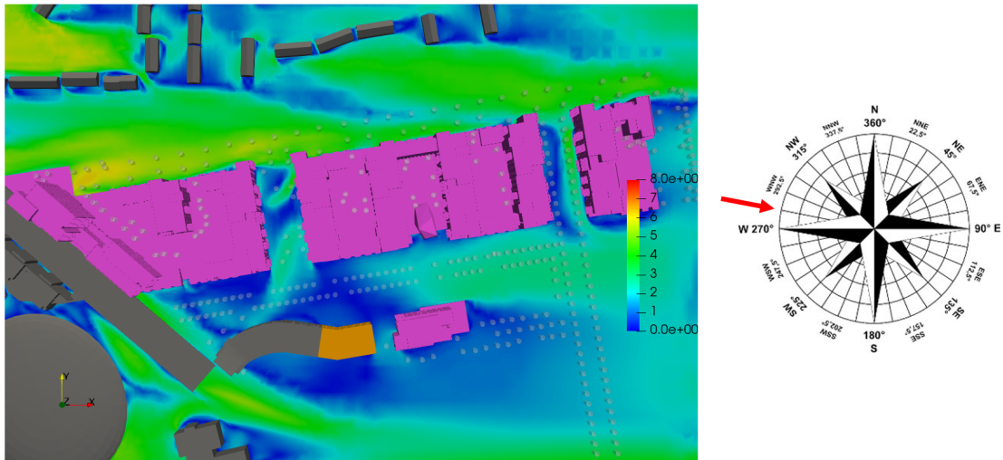
Figure 6.20: Ground Floor Level - Flow Velocity Results at Z=1.5m above the ground including existing buildings (in grey) and permitted but not constructed (in orange) - Wind Direction: 281°
