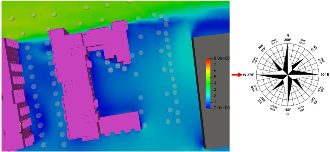
Figure 6.43: Block F Podium - Flow Velocity Results at Z=1.5m above the Podium - Wind Direction: 270°
