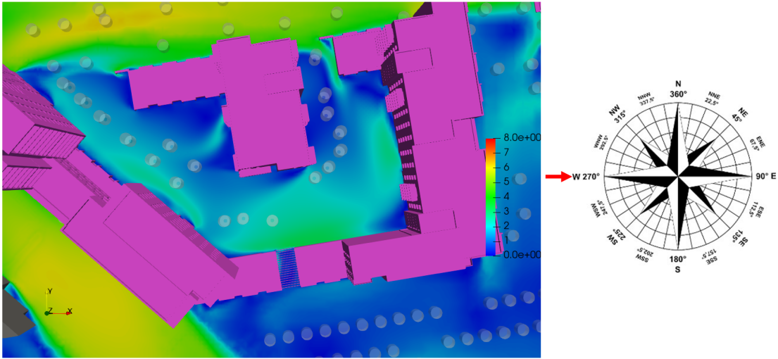
Figure 6.27: Block A/B/C Podium - Flow Velocity Results at Z=1.5m above the Podium - Wind Direction: 270°
