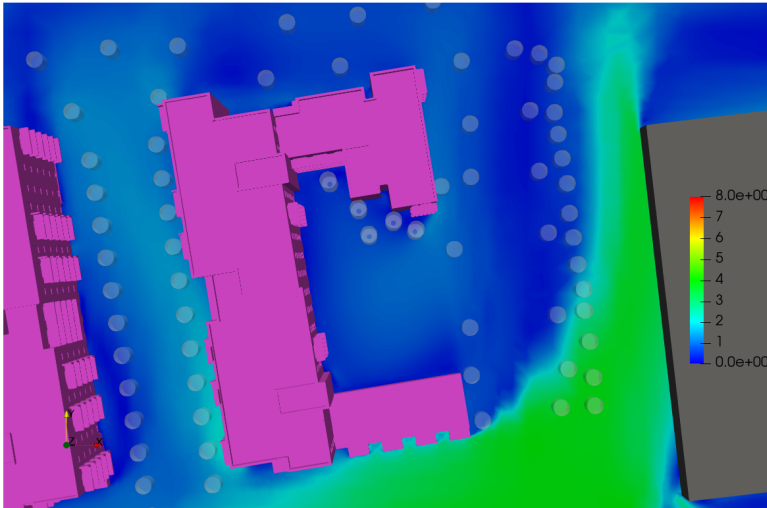
Figure 6.38: Block F Podium - Flow Velocity Results at Z=1.5m above the Podium - Wind Direction: 225°
