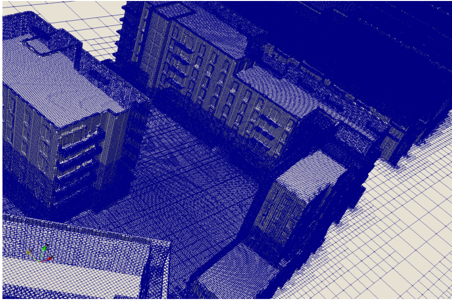
Figure 4.2: Park West SHD Domain Computational Mesh Utilized
