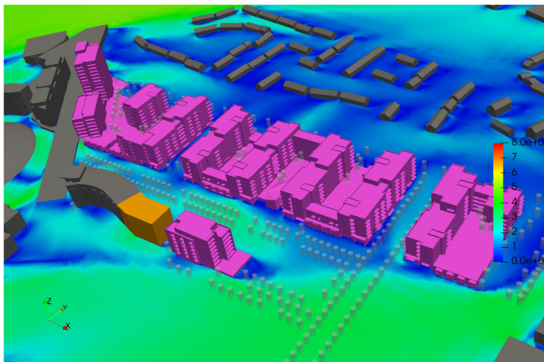
Figure 6.7: Wind Speed Results at 1.5m Above Development Ground Floor including existing buildings (in grey) and permitted but not constructed (in orange) - 3D View - Wind Direction: 225°
