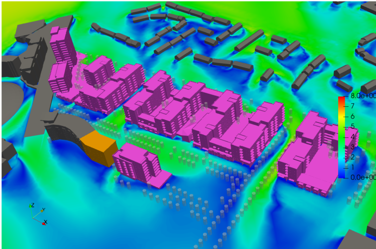
Figure 6.19: Wind Speed Results at 1.5m Above Development Ground Floor including existing buildings (in grey) and permitted but not constructed (in orange) - 3D View - Wind Direction: 315°
