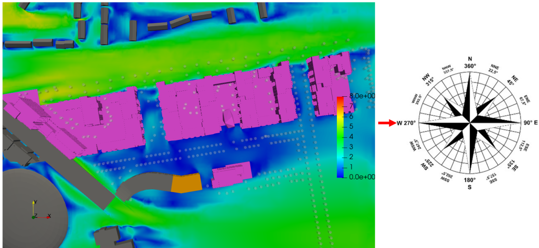
Figure 6.16: Ground Floor Level - Flow Velocity Results at Z=1.5m above the ground including existing buildings (in grey) and permitted but not constructed (in orange) - Wind Direction: 270°
