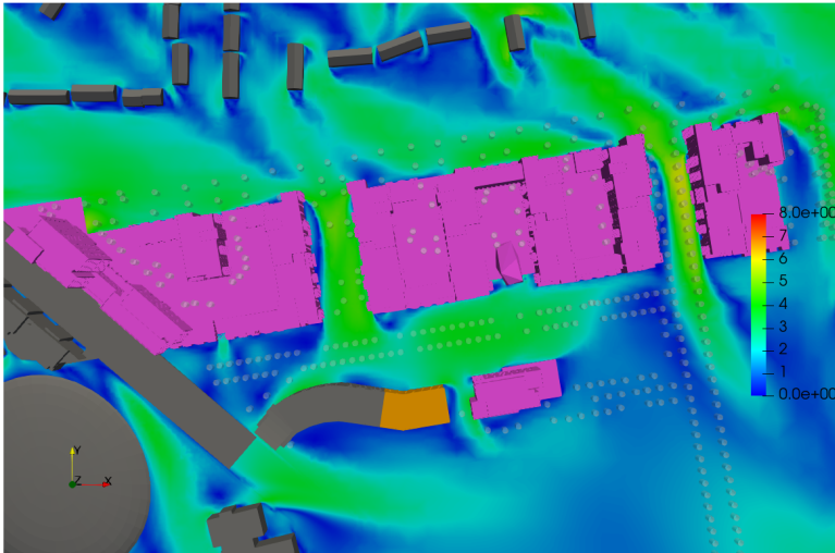
Figure 6.18: Ground Floor Level - Flow Velocity Results at Z=1.5m above the ground including existing buildings (in grey) and permitted but not constructed (in orange) - Wind Direction: 315°
