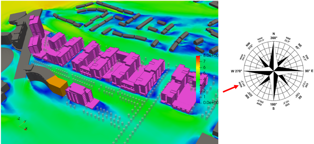
Figure 6.15: Wind Speed Results at 1.5m Above Development Ground Floor including existing buildings (in grey) and permitted but not constructed (in orange) - 3D View - Wind Direction: 247°
