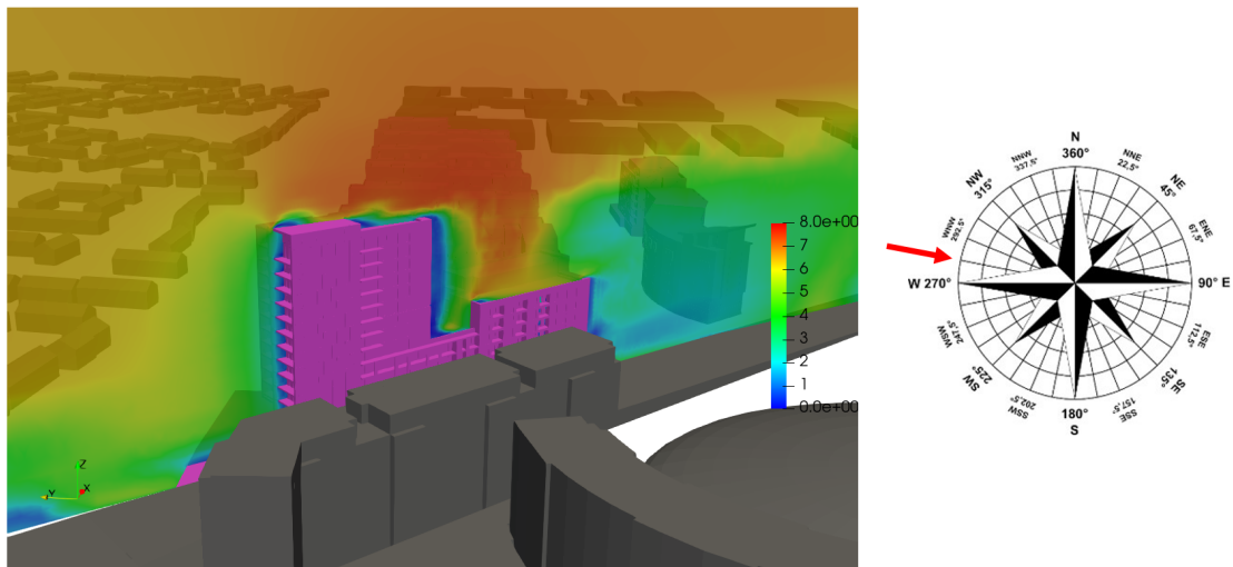
Figure 6.61: Flow Velocity Results of some balconies on the tallest building of the development - Wind Direction: 281°
