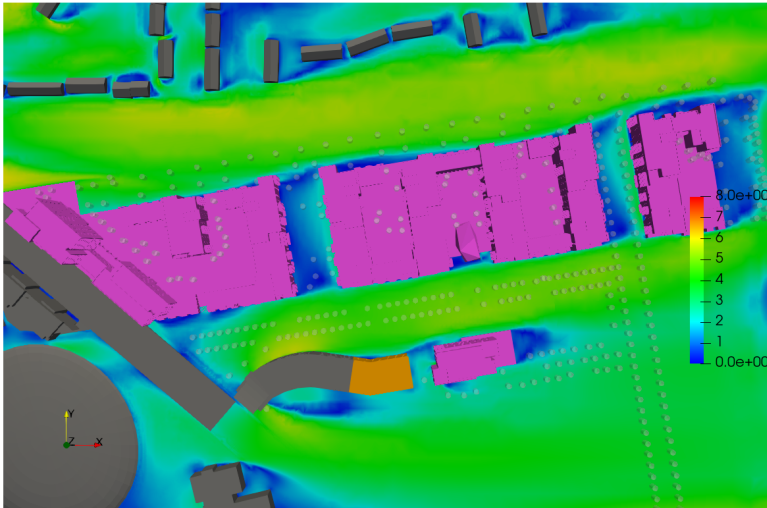
Figure 6.12: Ground Floor Level - Flow Velocity Results at Z=1.5m above the ground including existing buildings (in grey) and permitted but not constructed (in orange) - Wind Direction: 258°
