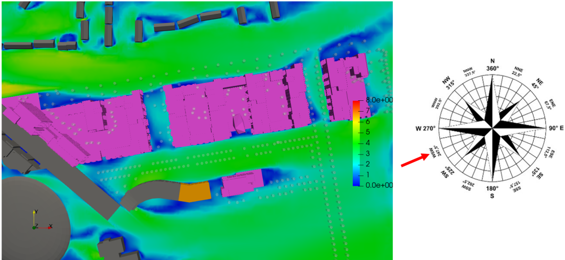
Figure 6.14: Ground Floor Level - Flow Velocity Results at Z=1.5m above the ground including existing buildings (in grey) and permitted but not constructed (in orange) - Wind Direction: 247°
