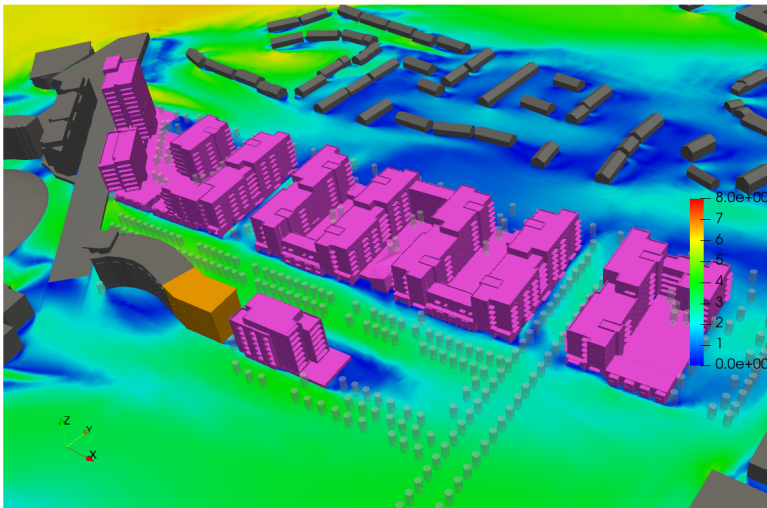
Figure 6.11: Wind Speed Results at 1.5m Above Development Ground Floor including existing buildings (in grey) and permitted but not constructed (in orange) - 3D View - Wind Direction: 236°
