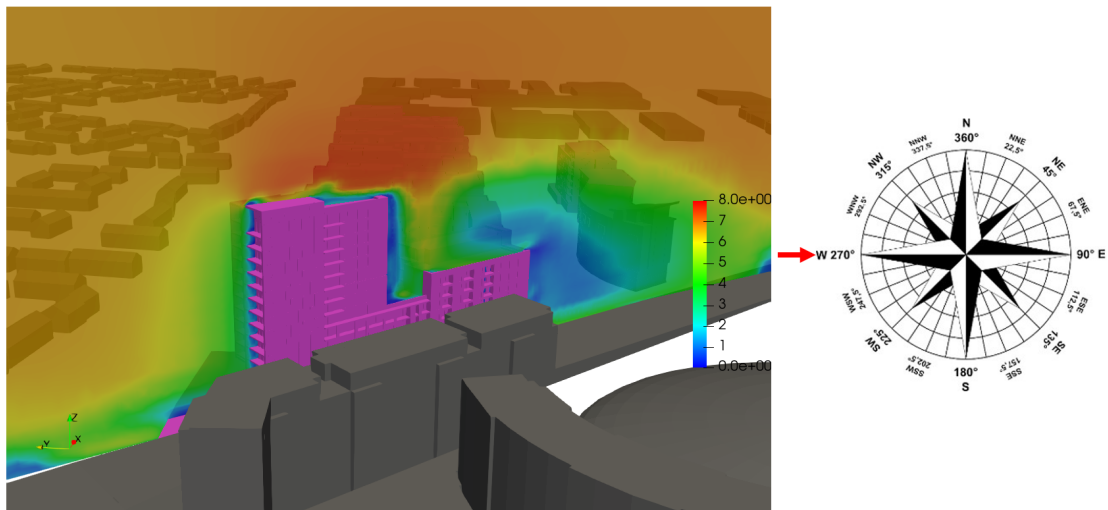
Figure 6.57: Flow Velocity Results of some balconies on the tallest building of the development - Wind Direction: 270°
