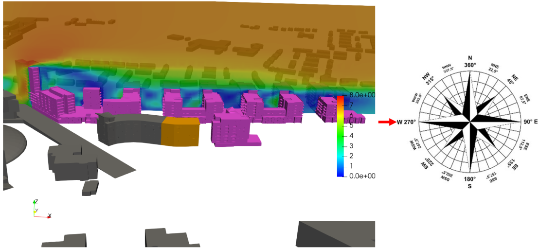
Figure 6.56: Flow Velocity Results of some balconies on the West/East sides of the development - Wind Direction: 270°
