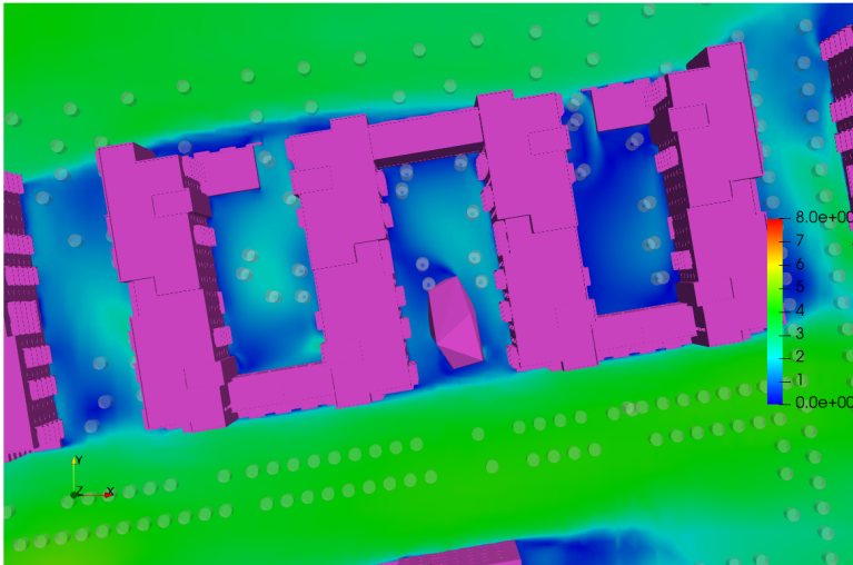
Figure 6.34: Block D/E Podium - Flow Velocity Results at Z=1.5m above the Podium - Wind Direction: 247°
