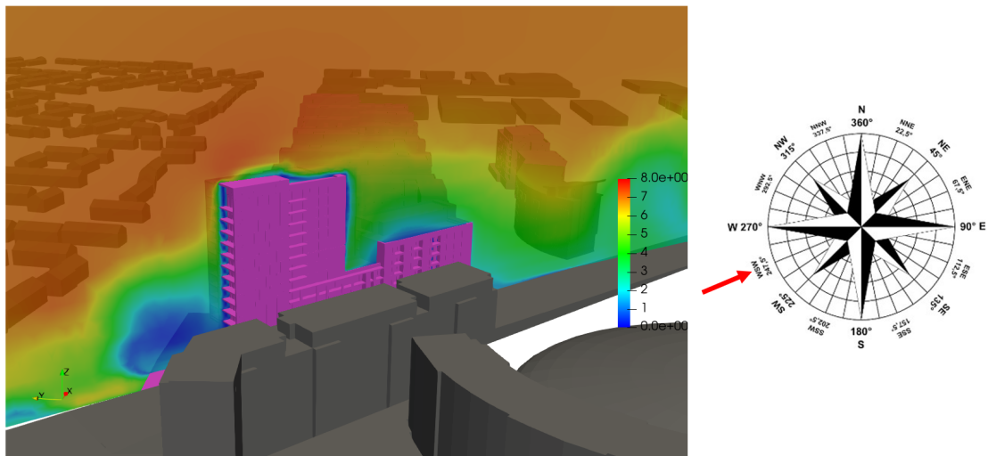
Figure 6.55: Flow Velocity Results of some balconies on the tallest building of the development - Wind Direction: 247°
