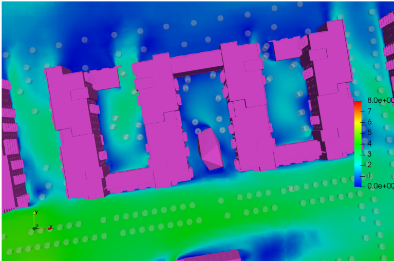
Figure 6.32: Block D/E Podium - Flow Velocity Results at Z=1.5m above the Podium - Wind Direction: 236°
