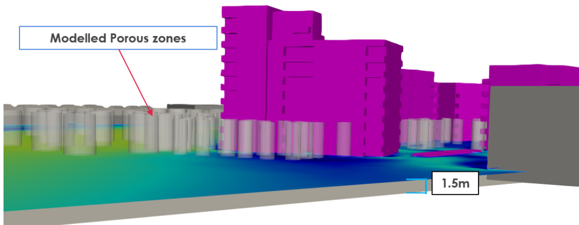
Figure 6.5: An example of wind data mapped on surface at 1.5m above the ground
