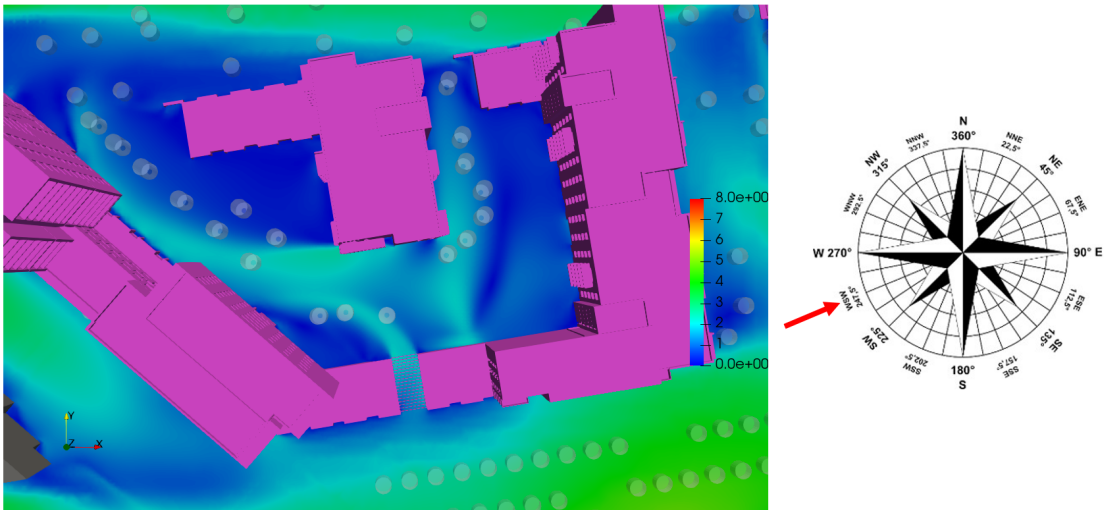
Figure 6.26: Block A/B/C Podium - Flow Velocity Results at Z=1.5m above the Podium - Wind Direction: 247°
