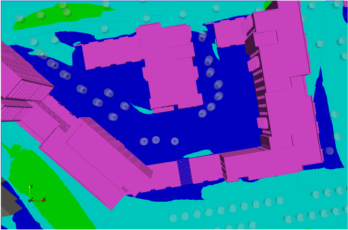
Figure 6.65: Block A/B/C Podium - Lawson Discomfort Map - Top View
