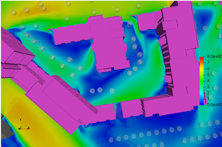
Figure 6.29: Block A/B/C Podium - Flow Velocity Results at Z=1.5m above the Podium - Wind Direction: 281°
