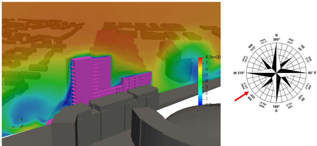
Figure 6.51: Flow Velocity Results of some balconies on the tallest building of the development - Wind Direction: 236°
